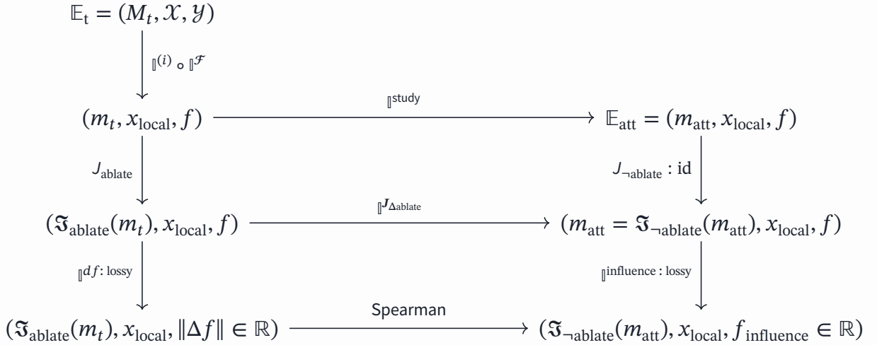
Figure 10: No estimate node-logit influence, the paper ablates the target world but not the proxy world. By this construction, \mathbb{J}^{J_{\Delta\text{ablate}}} will encode the magnitude of its effect 46 . To approximate it, the authors study the world-to-world correlation from re-interpreted versions. The re-interpretations are technically lossy but useful to compute an actual number.
