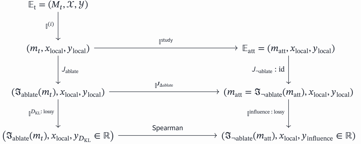
Figure 10: No estimate node-logit influence, the paper ablates the target world but not the proxy world. By this construction, \mathbb{J}^{J_{\Delta\text{ablate}}} will encode the magnitude of its effect 46 . To approximate it, the authors study the world-to-world correlation from re-interpreted versions. The re-interpretations are technically lossy but useful to compute an actual number.
